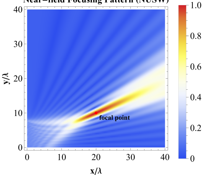
Near-field Focusing Pattern (NUSW)
